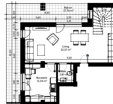
PLAN PARTER
