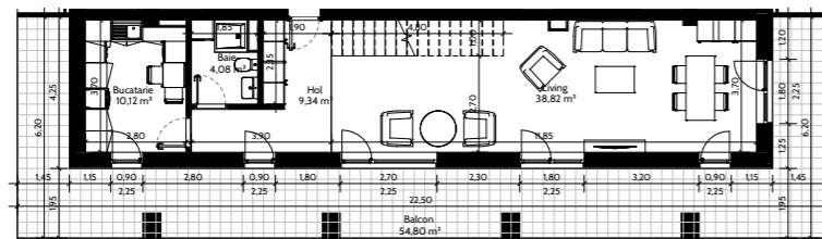
PLAN PARTER
